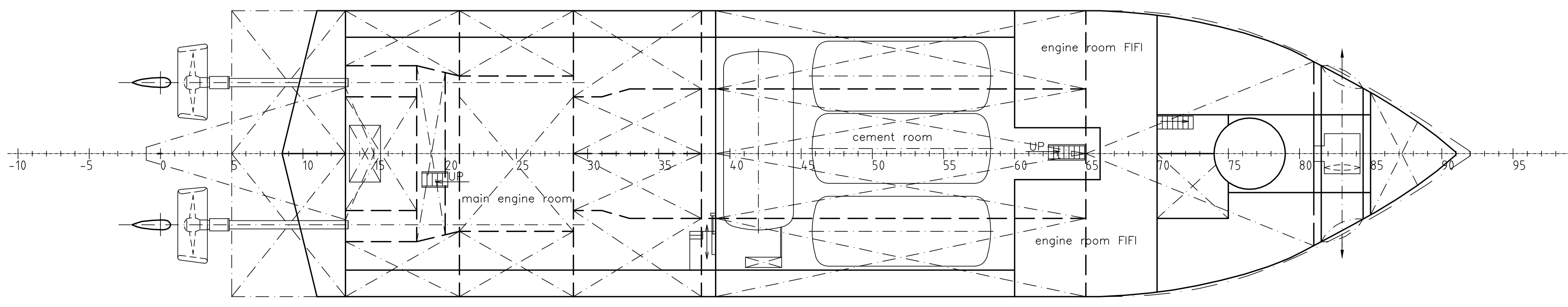
TANKTOP
